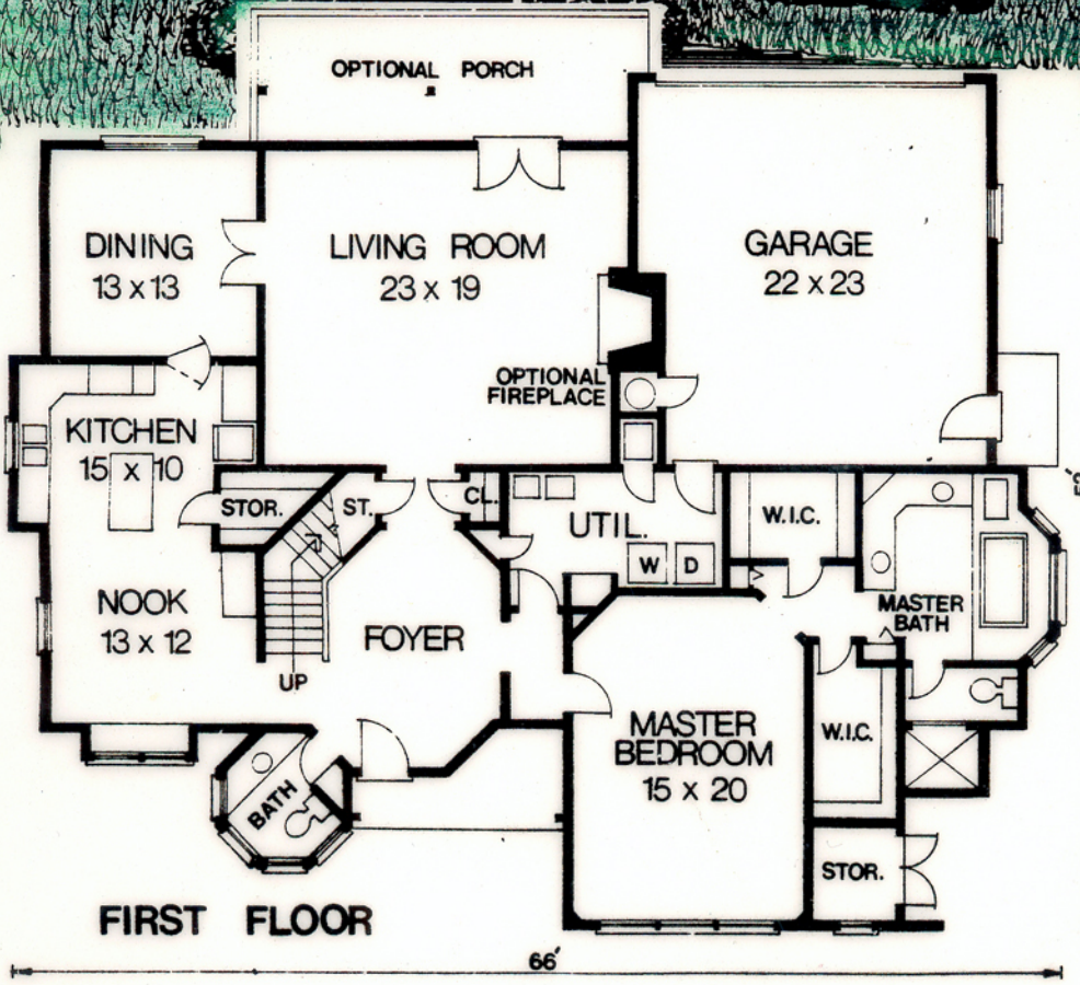
MAIN LEVEL Living area: 2,250 s.f. Garage: 528 s.f.
