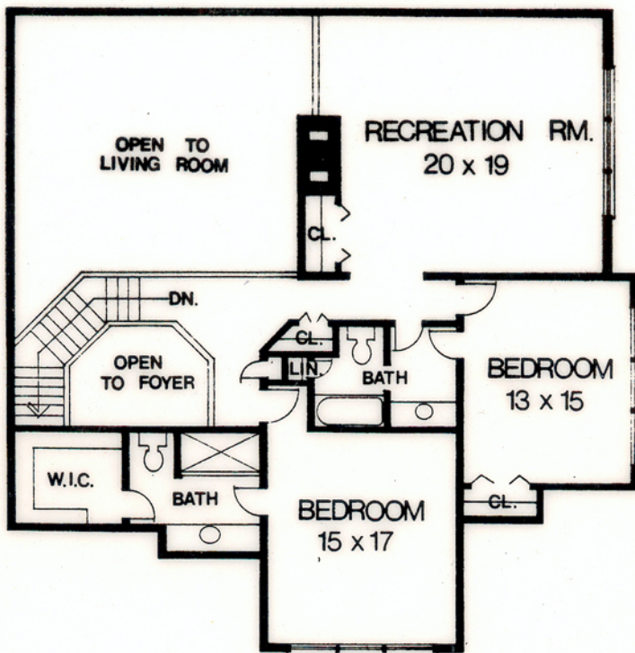
UPPER LEVEL Living area: 1,550 s.f.
